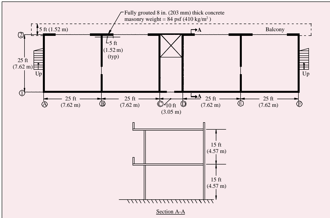
Figure 4—Example Masonry Building
