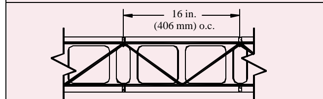
Figure 2—Truss-Type Joint Reinforcement
